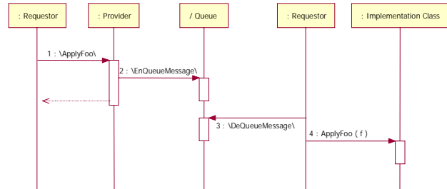
Figure 12 – Queued implementation
