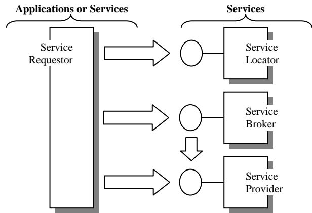
Figure 1 – Service terminology
