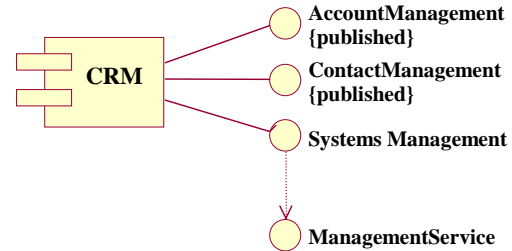
Figure 2 – Implemented services
