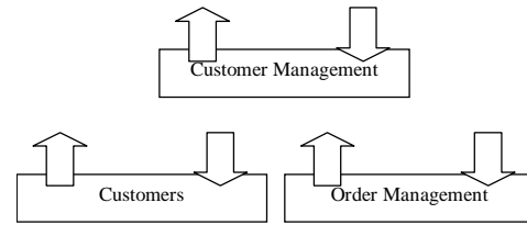
Figure 10 – Service dependencies
