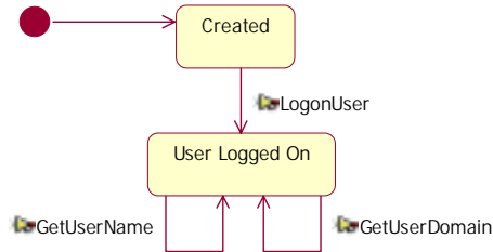
Figure 4 – Interface behavior
